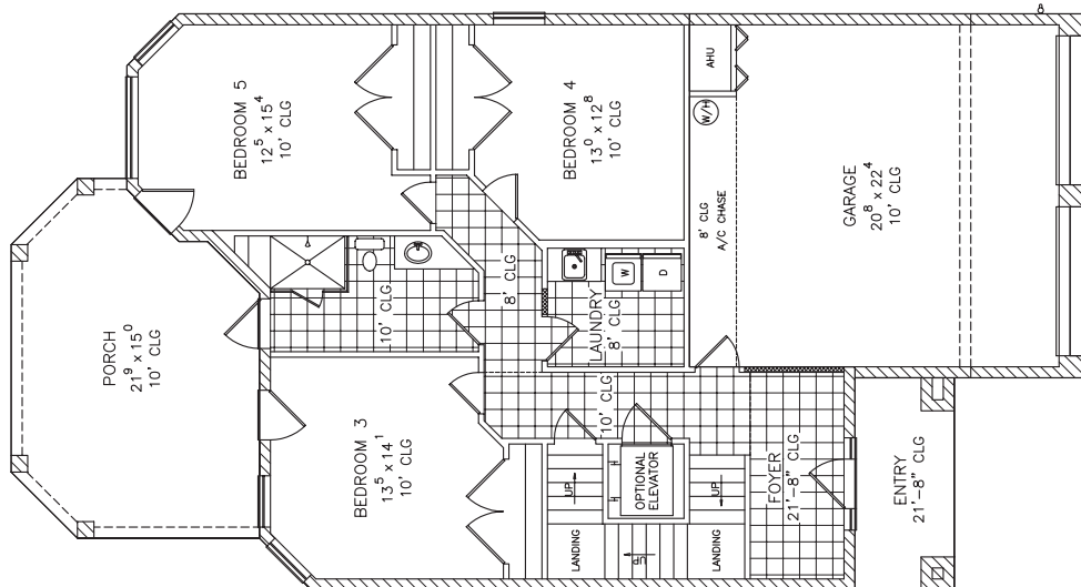
1st FLOOR
