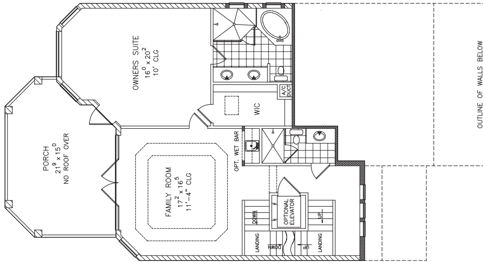
3rd FLOOR
