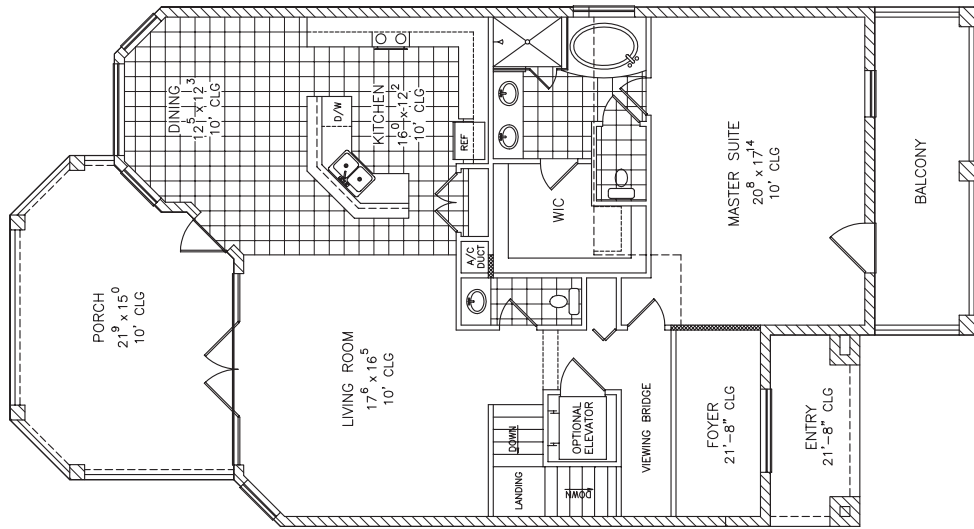
2nd FLOOR
