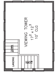
TOWER PLAN
